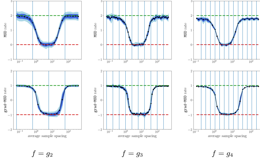
Figure 4: We examine the effect of stepping up the input dimension for the Griewank function g_d : \mathbb{R}^d \rightarrow \mathbb{R} , given in Eq. (3). We fix query points \{q_i\} and a bounding box \mathcal{B} , centered at the origin, then run distinct experiments by scaling both by pre-determined amounts. Vertical blue bars separate the distinct scales of experiments. As the dimension increases, we use more distinct scales with fewer iterations per scale, demonstrating one approach for scaling with dimension. The computed rates have the same behavior in each dimension, further validating the method.
