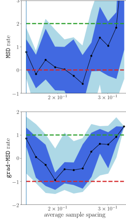
Figure 5: We apply Algorithm 4 to a static dataset of 13,016 data points gathered from simulations of internal confinement fusion, produced by the HYDRA codebase. The computed rates suggest that the data set has small scale geometric features, since the grad-MSD rate is nearly equal to the recoverable feature (i.e., 1) at the smallest possible <samp> value. Decreasing <samp> further would require generating more data, demonstrating how the Delaunay density diagnostic can be used to inform the need for data collection.
