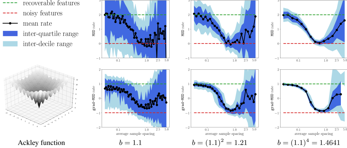
Figure 3: For the Ackley function on \mathbb{R}^2 —shown at left—we examine the effect of changing the upsampling rate b on the rates computed by Algorithm 2 and Algorithm 3. Using the values of b indicated, we confirm that a larger b value corresponds to a larger step size (in the horizontal axis) and a smaller variation in the computed rate, as evidenced by the narrower inter-quartile and inter-decile ranges as b increases. For larger average sample spacings, the small number of samples is the cause of the increased variation. In each case, the mean rate has the same trend, reflecting the multi-scale nature of the Ackley function.
