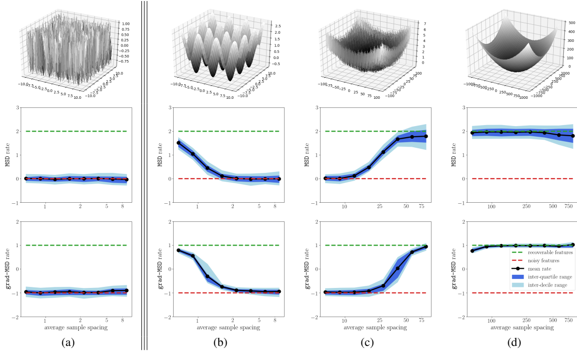
Figure 2: We validate Algorithm 2 and Algorithm 3 by assessing the computed rate over a range of average sample spacings, for f shown in the top row. The mean rate (black dot series) shows the average of the computed rate over 100 trials with different random initial seeds. (a) Pure noise is consistently detected as having the “noisy features” rate (0 for MSD, -1 for grad-MSD). (b) Fine scale features are only recoverable if average sample spacing is small enough. (c) Insufficiently sampled fine scale features are detected as noise; the large scale quadratic feature is recoverable with larger average sample spacing. (d) Smooth variation (at the scale of inquiry) is consistently detected as having the “recoverable features” rate (2 for MSD, 1 for grad-MSD).
